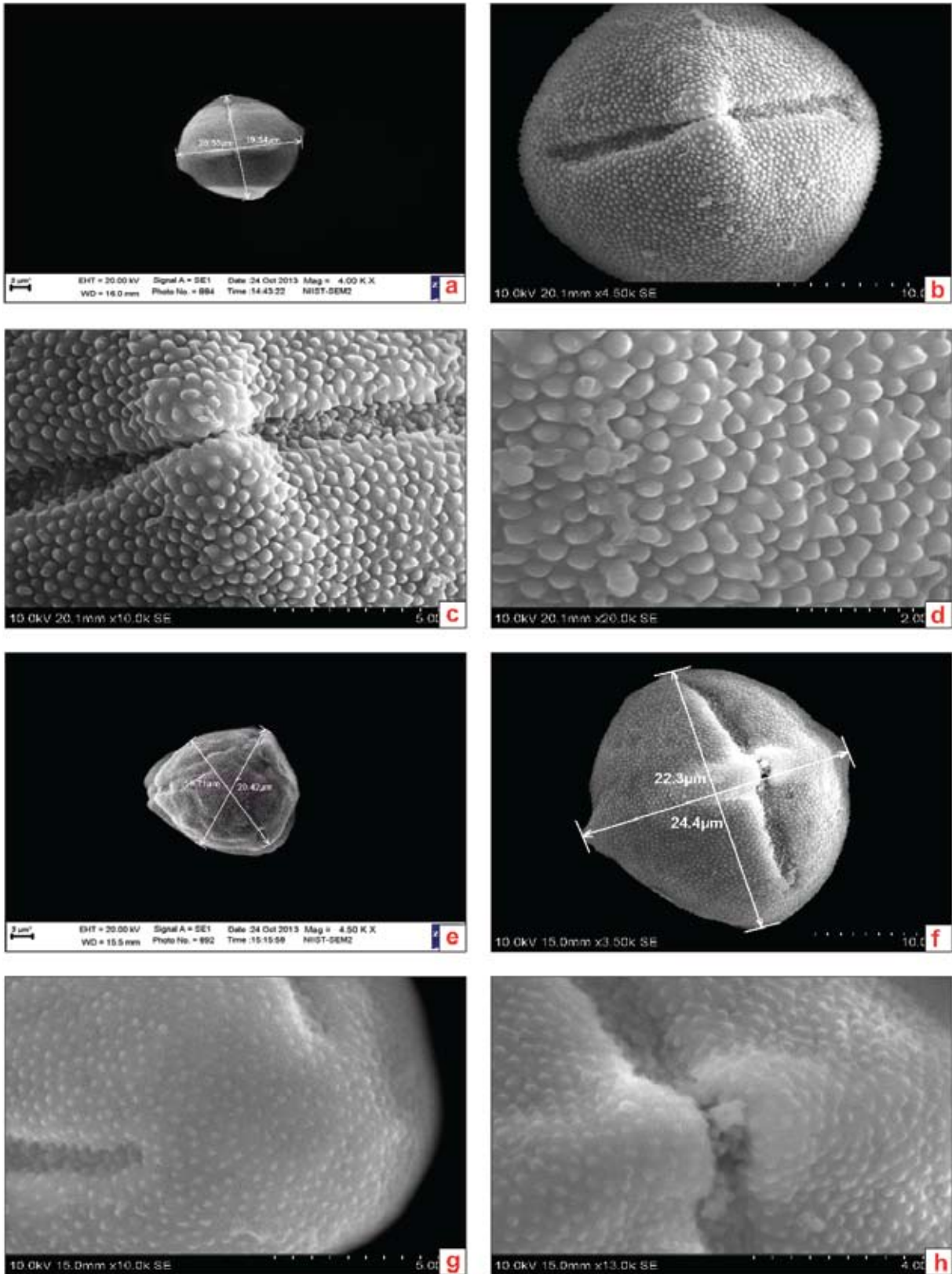
Fig. 9. a–d. Solanum macrocarpon L.: a. Equatorial view; b. colpus with ridge at the pore., c & d. exine ornamentation. e–h. Solanum mammosum L.: e. Polar view; f. Equatorial view; g. Apocolpium region; h. Colpus region.
