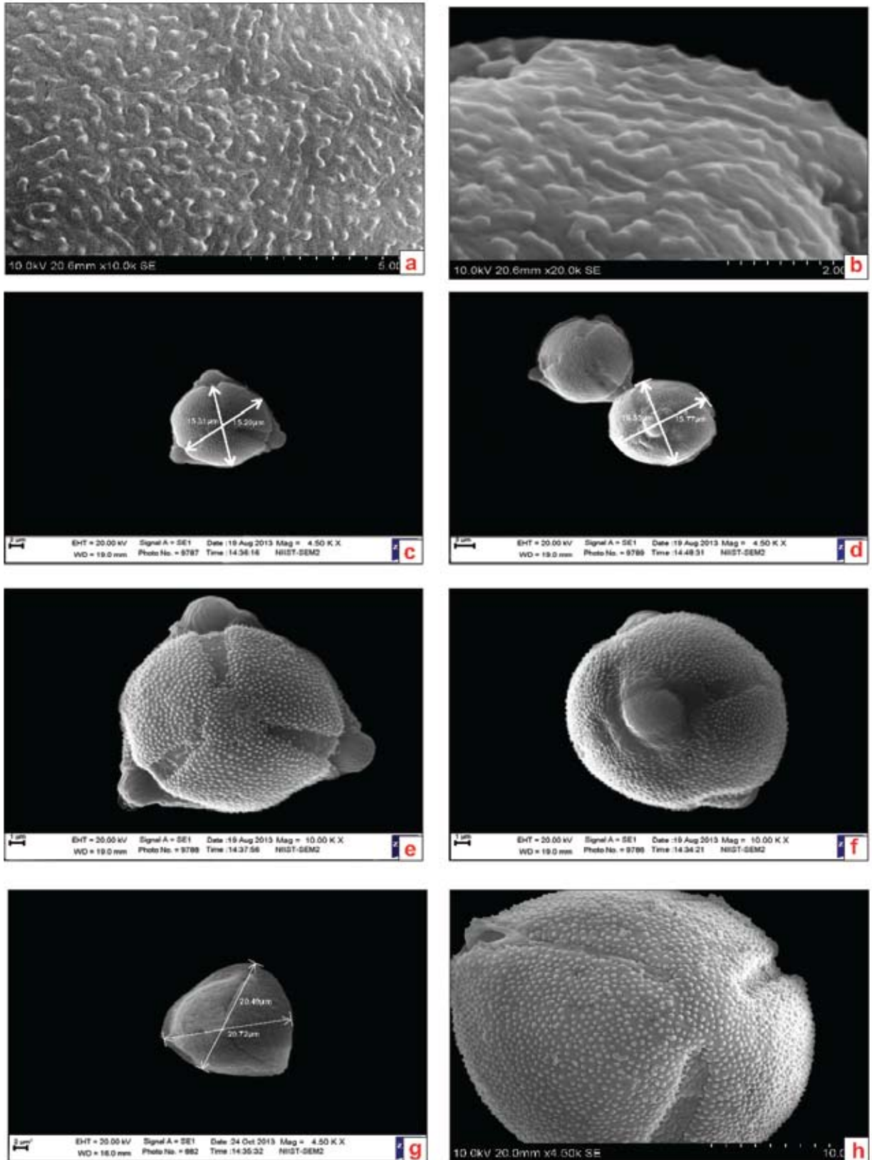
Fig. 8. a & b. Solanum violaceum Ortega. subsp. violaceum : a. Apocolpium showing triplex joining of elements; b. Ornamentation at mesocolpium. c–f. Solanum wendlandii Hook: c. Polar view; d. Equatorial view; e. Compact spinulose exine ornamentation; f. Globose operculum and multi bridging at the colpus., g & h. Solanum macrocarpon L.: g. Polar view; h. Apocolpium view.
