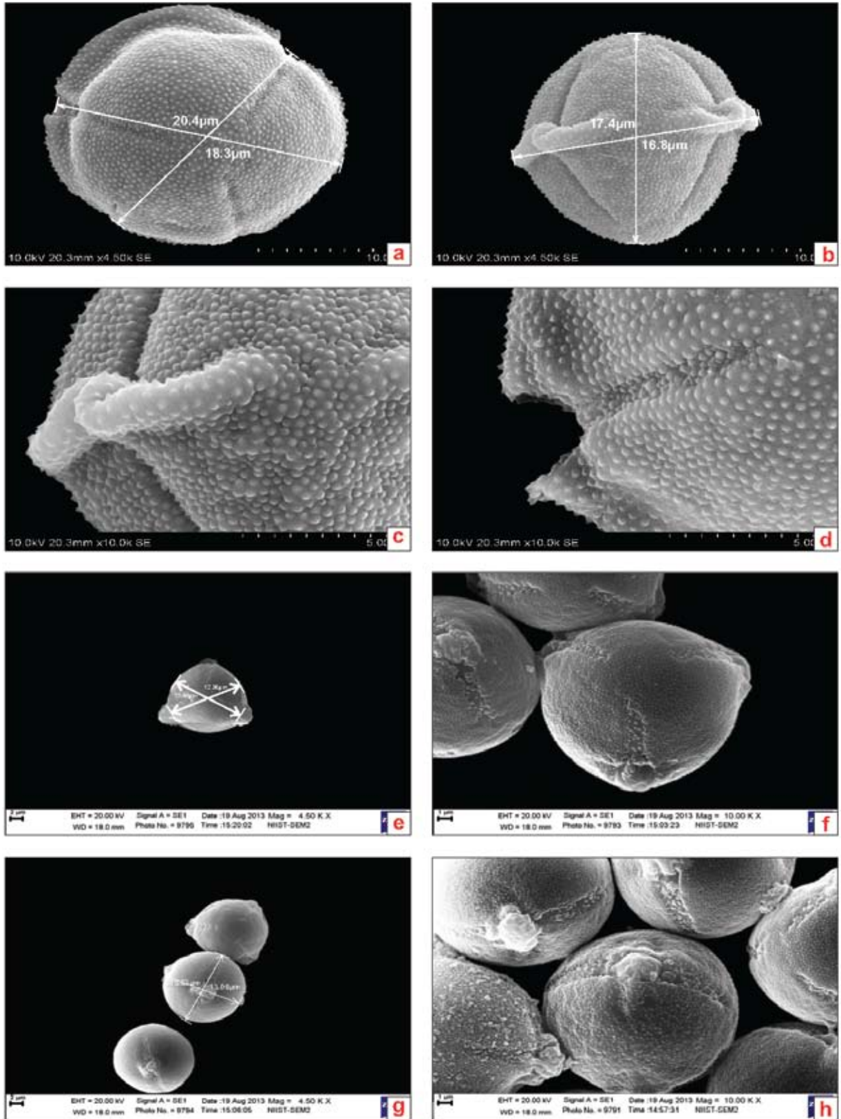
Fig.1. a–d. Solanum aculeatissimum Jacq.: a. Polar view; b. Equatorial view; c. Ornamented operculum; d. Exine ornamentation., e–h. Solanum americanum Mill.: e. Polar view; f. Microechinate exine; g. Equatorial view; h. Colpus showing minute granules.
